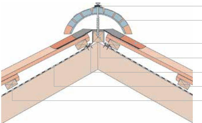
Typical example – hip detail with universal hip tiles
