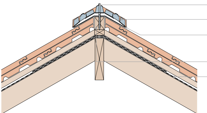
Typical example – hip detail with universal hip tiles
